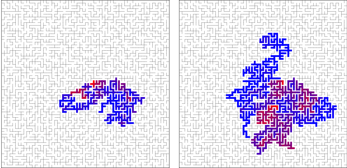
Figure 1: The range of a realisation of the simple random walk on uniform spanning tree on a 60 \times 60 box (with wired boundary conditions), shown after 5,000 and 50,000 steps. From most to least crossed edges, colours blend from red to blue.
