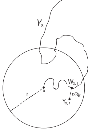
Figure 2: A sample of A_1(x, r, k) in Lemma 2.5.
