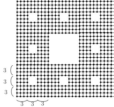
Figure 2: The Sierpinski carpet graph.
